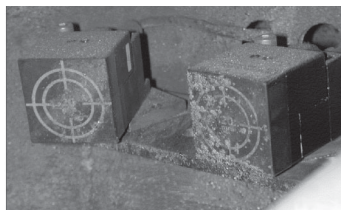
Standard Sensor Failed due to weld slag adhesion after 1,663 Weld Cycles
